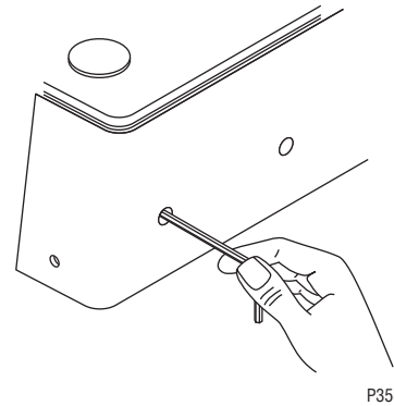
FIG 16 Adjusting Water Flow Using 1/4" allen wrench
